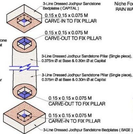
ISOMETRIC VIEW SHOWING MALE-FEMALE PILLAR JOINT AT CAPITAL & BASE
