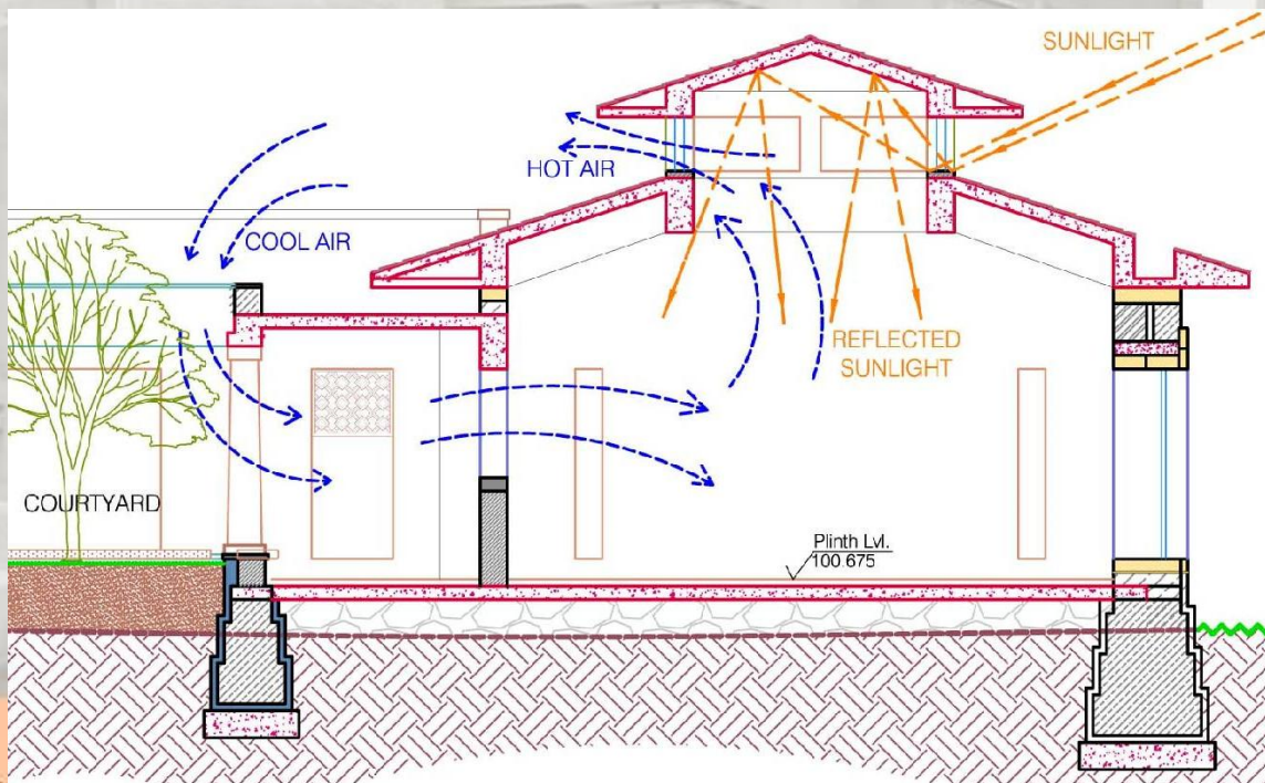
SECTION THROUGH COURTYARD CLASSROOM BLOCK
