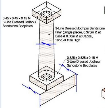
ISOMETRIC VIEW OF ROUND SANDSTONE PILLARS AT BARADARI
