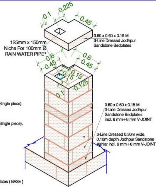
ISOMETRIC VIEW OF CORNER SANDSTONE MASONRY PILLARS AT BARADARI
