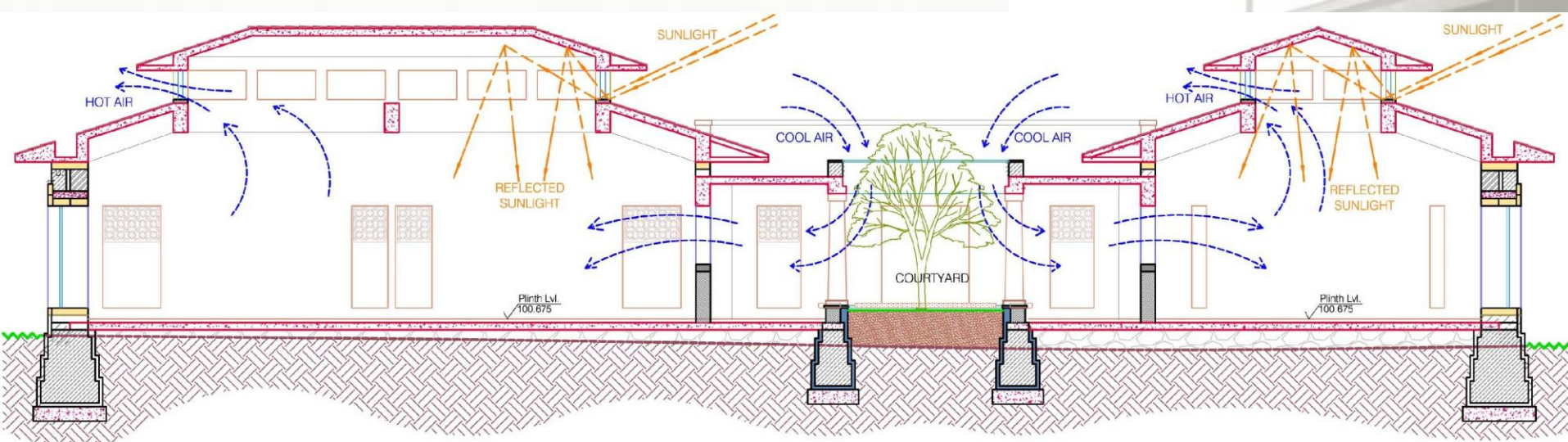
SECTION THROUGH COURTYARD CLASSROOM BLOCK
