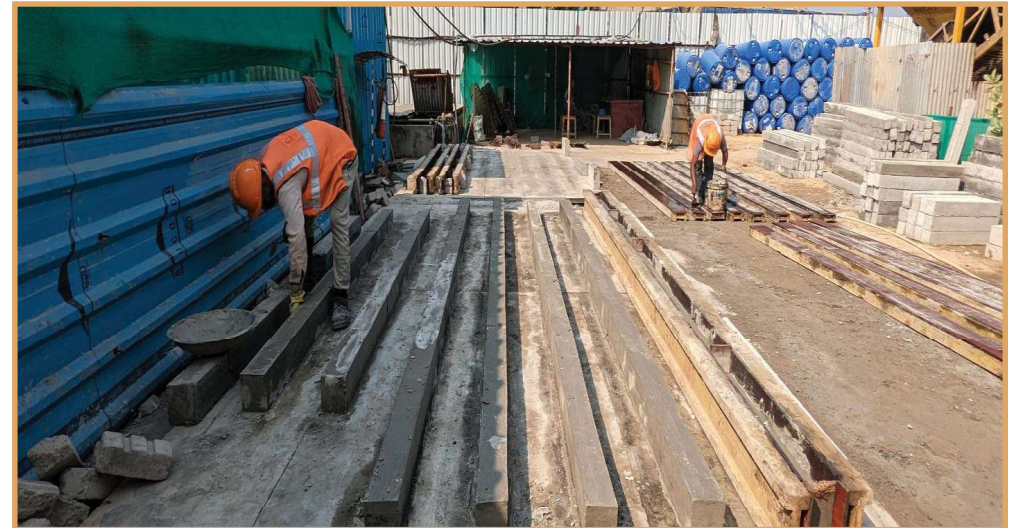
▲ Demonstration of reuse of waste concrete used on site to make lintels
