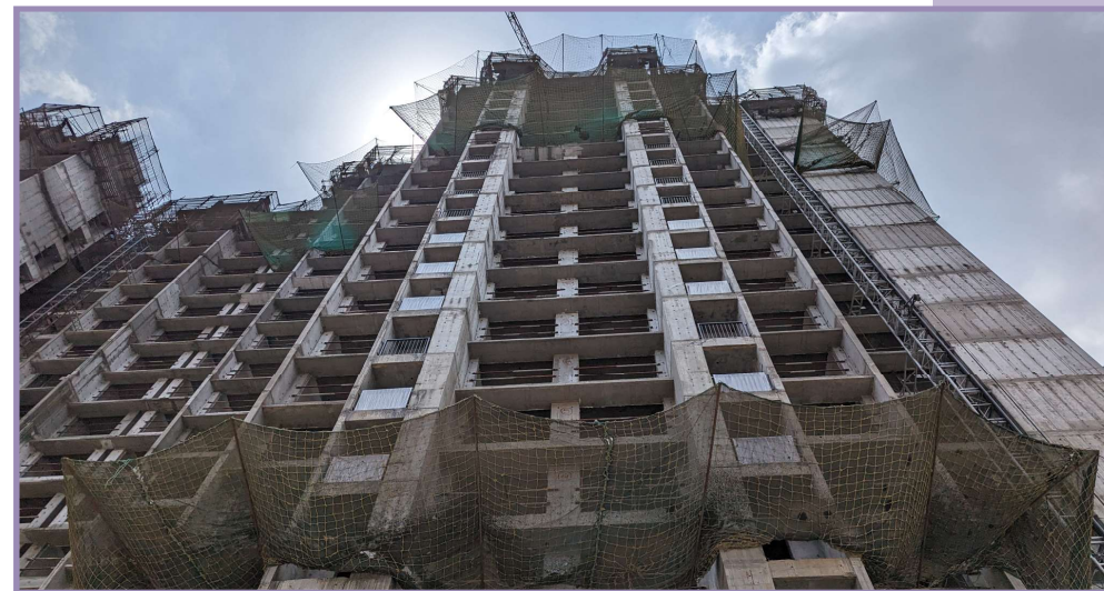
▲ Provision of safety nets for a multi-storey building under construction
