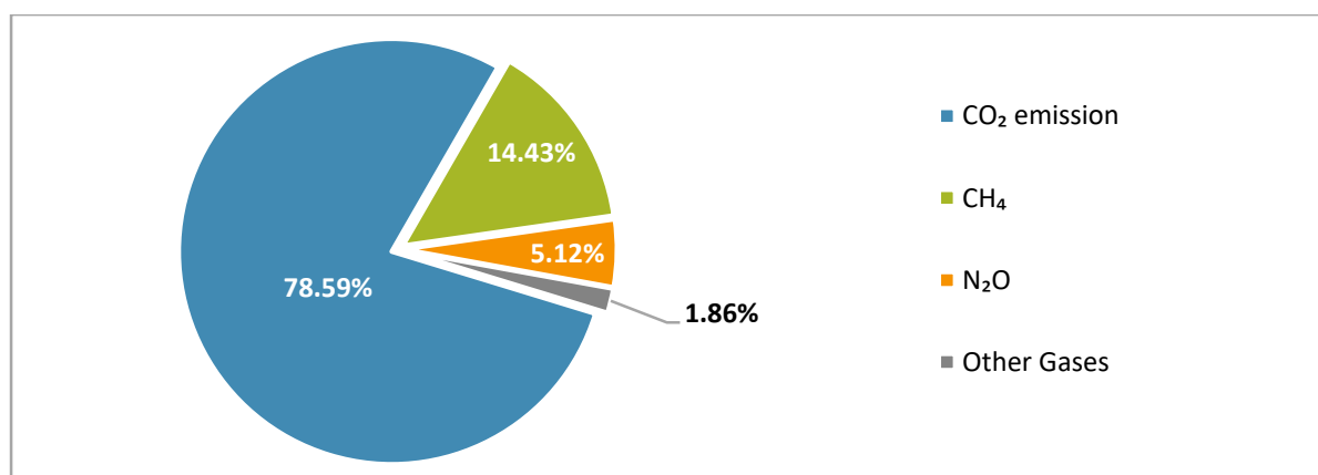
Figure 2.6: Gas-wise emission for the year 2016
