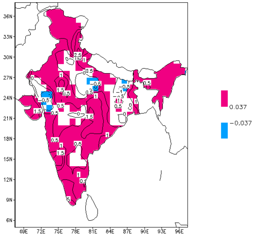
Figure 1.4: Annual mean temperature anomaly trends (°C /100 years) are shown as contour lines. The trends significant at the 95% level are shaded. Positive trends are shown in red while the negative trends are shown in blue. Period of analysis: 1901–2019. (Departure from 1981-2010 average). Source: IMD, 2020.
