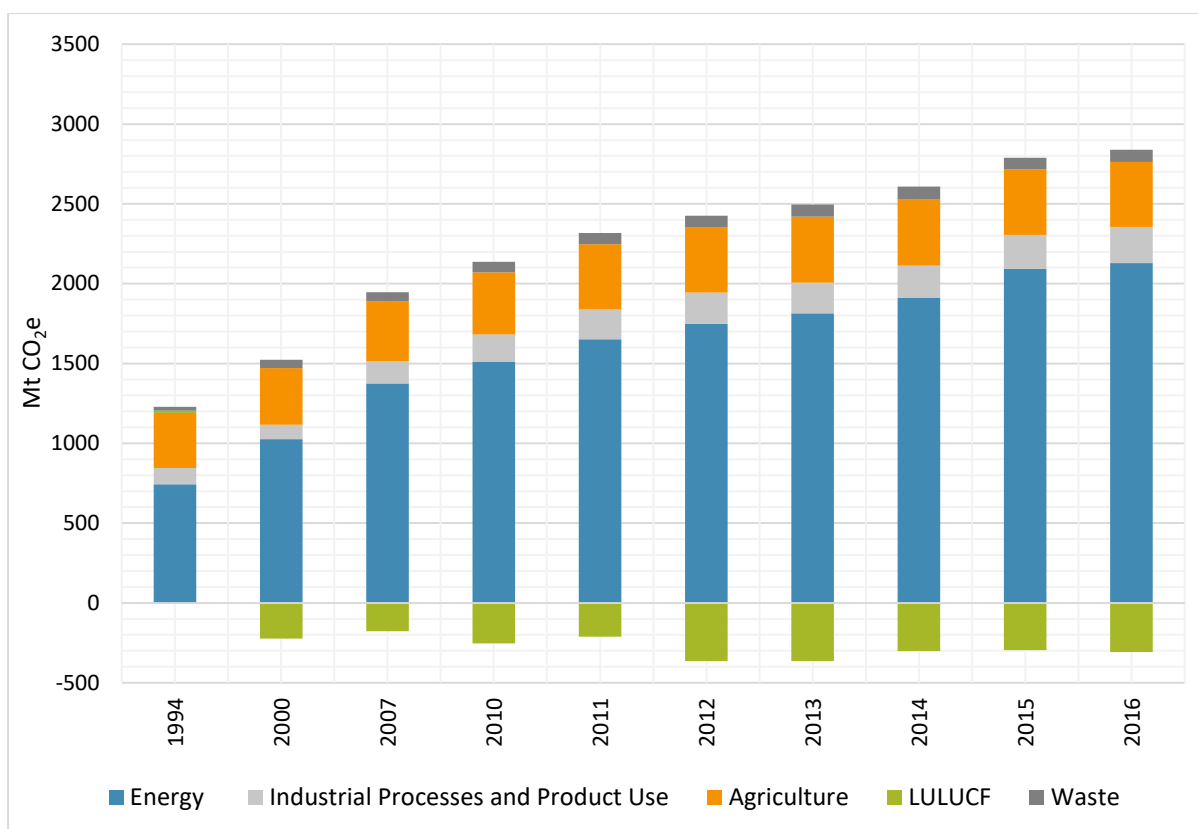
Figure 2.2: Sector-wise National GHG emission in Mt CO 2 e for 1994-2016.
