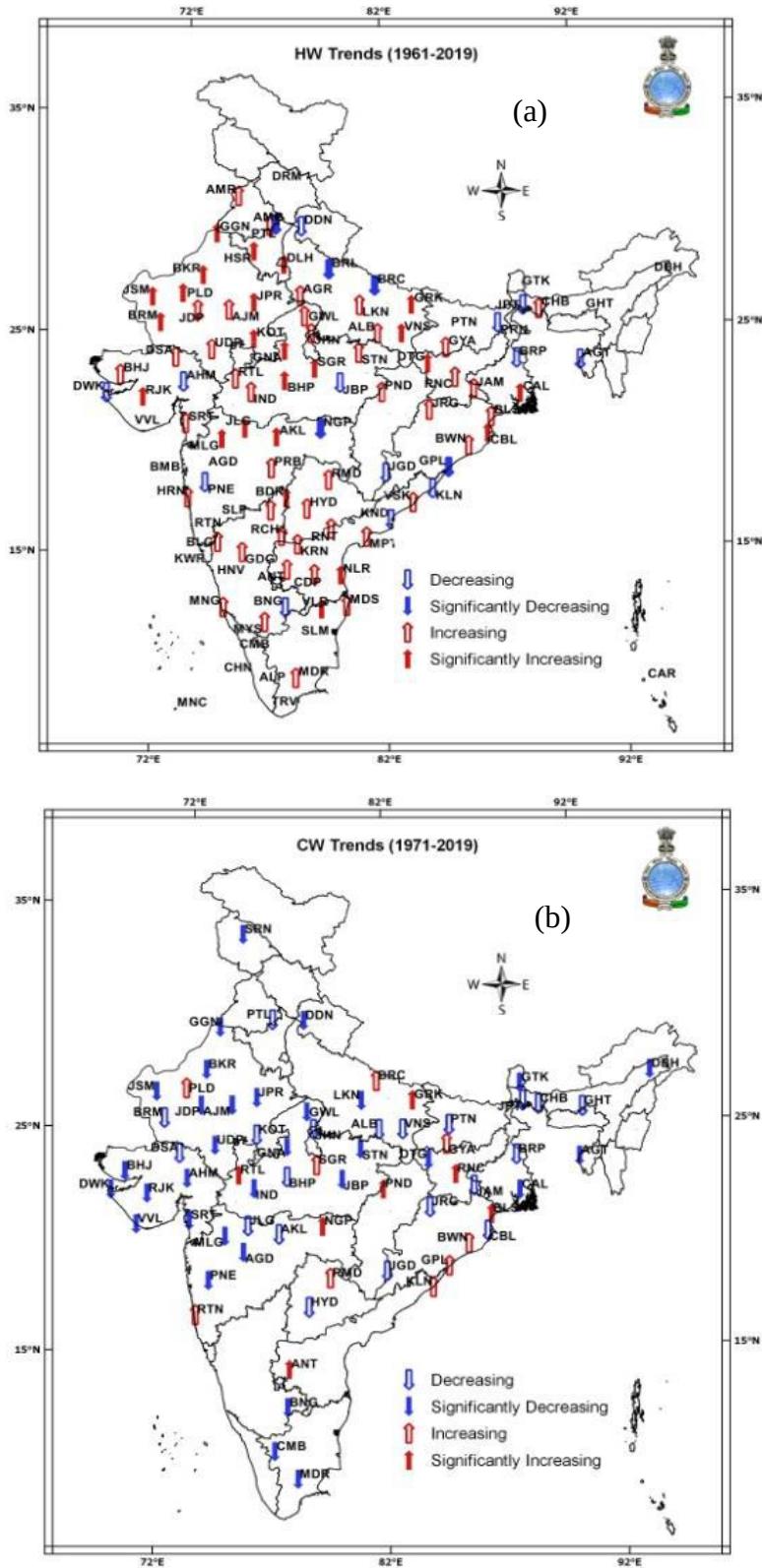
Figure 1.7: (a) Trends in the Heat Wave (HW) days of 103 stations during April, May and June for the period 1961–2019. (b) Trends in the Cold Wave (CW) days of 86 stations during the December, January and February for the period 1971–2019. Nonparametric Mann–Kendall test was used to test the significance of the trends. Source: IMD, 2020.
